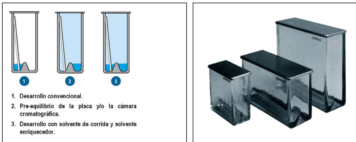
Figura 12.12. Twin Through Chamber
