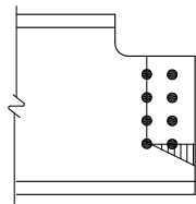
Multiple-Row Beam-End Connections
