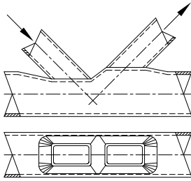
(a) Chord plastification
