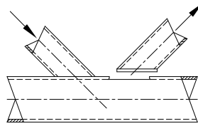
(b) Punching shear failure of chord
